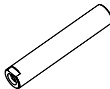
PART #66-SHAFT PIN, 1PCS. \Phi 25.4 \times 137 \text{mm}
