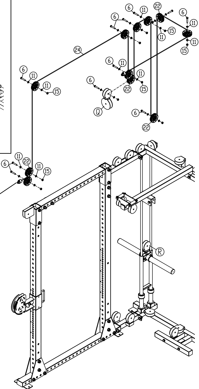
Above shows Step 6 assembled and completed.
