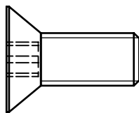
(A4)SOCKER FLAT HEAD SCREW M10X25L PARTIAL THREAD QTY.2
