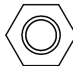
(A3)HEX BOLT M10X60L PARTIAL THREAD QTY.4
